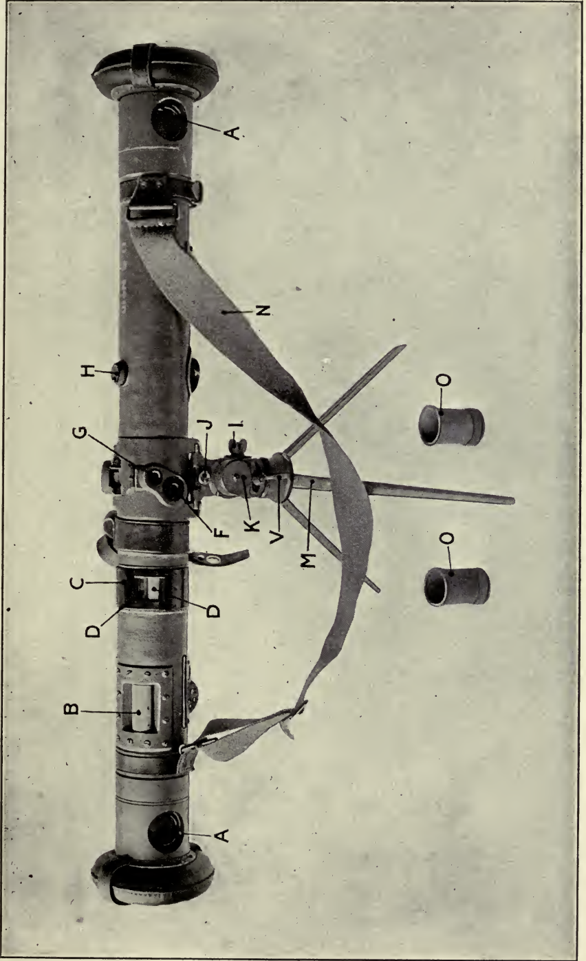
BAUSCH & LOMB, 70 CM. BASE, RANGE FINDER, FRONT VIEW.
